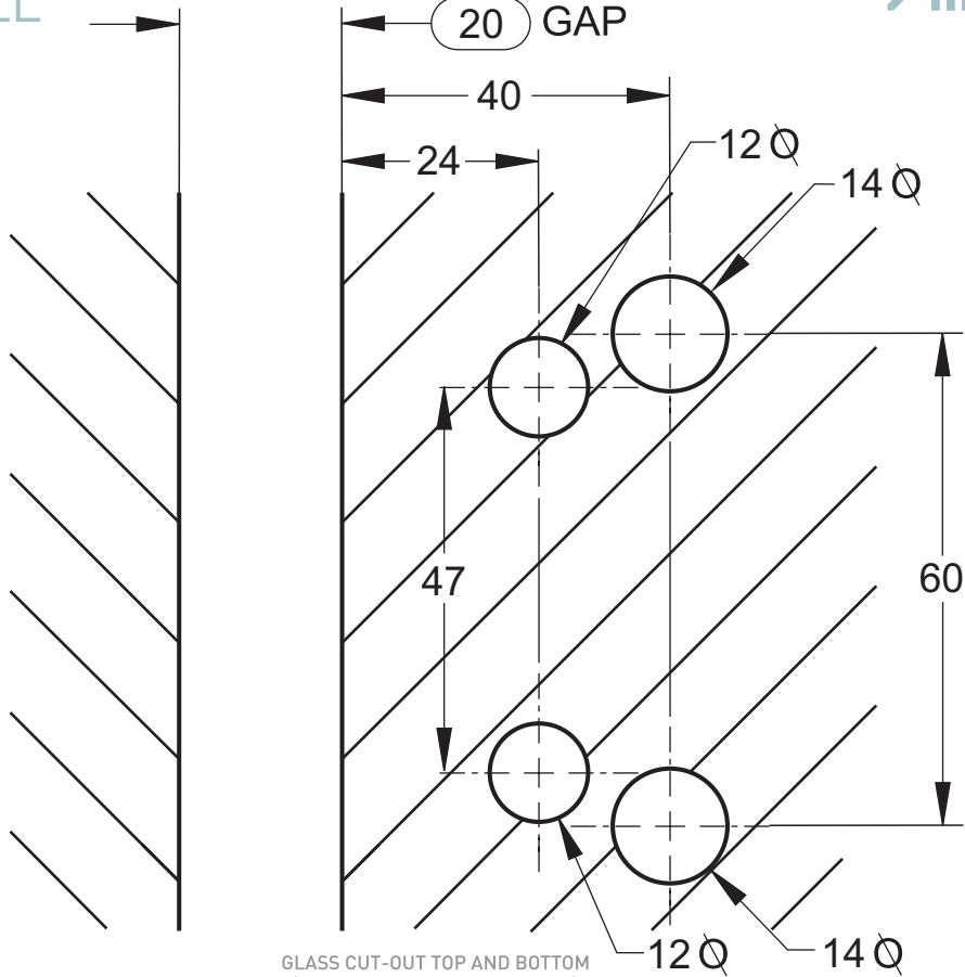
GLASS CUT-OUT TOP AND BOTTOM (ALL DIMENSIONS IN MILLIMETERS)
