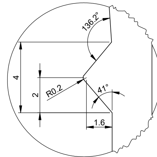
DETAIL C SCALE 7 : 1
