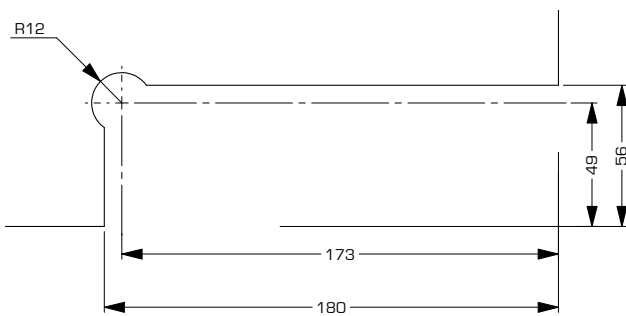
Glass detail
